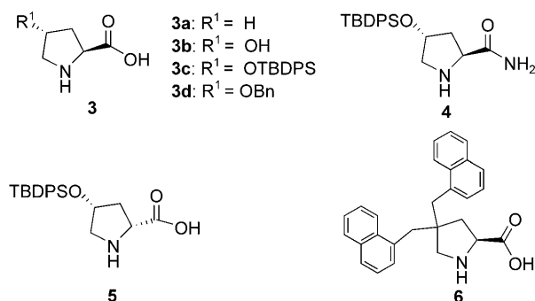
Scheme 1. Organocatalysts tested in this study.
