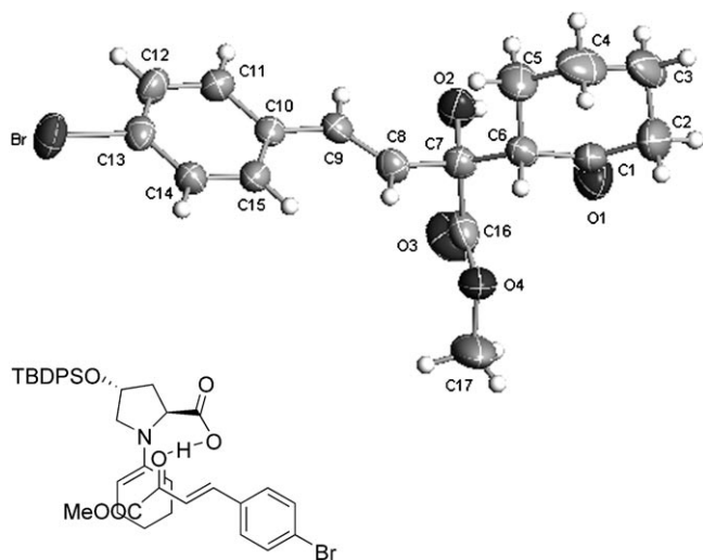
Figure 1. X-ray structure of adduct 2i and the proposed transition state.
