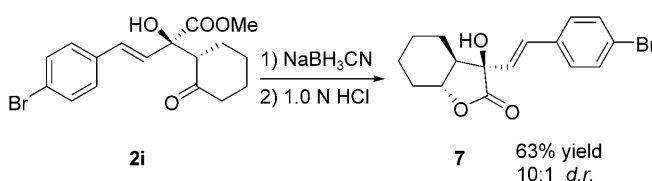
Scheme 2. Conversion of 2i to 7
